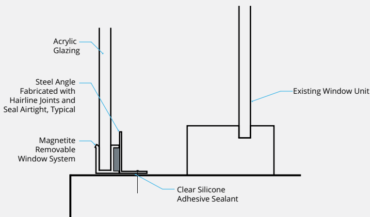
WINDOW DETAIL - SILL
